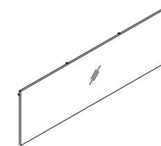
Clear Glass, Frosted Glass, Grey Glass 清玻璃·磨砂玻璃·灰玻璃 W: 400-1800 H: 300-450
