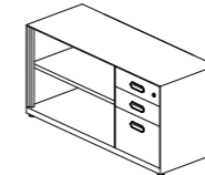
Fixed Return Combination Cabinet w/ Open Shelf & 3 Drawers 固定组合边柜，书架及三斗抽屉 W800 - W1600 x D450 x H710 (except W1300, W1500)
