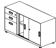
Mobile Return Combination Cabinet w/ Sliding Door & 3 Drawers 活动组合边柜，移门及三斗抽屉 W1100 - W1600 x D450 x H605 (except W1300, W1500)
