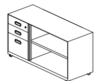
Mobile Return Combination Cabinet w/ Open Shelf & 3 Drawers 活动组合边柜，书架及三斗抽屉 W800 - W1600 x D450 x H605 (except W1300, W1500)
