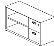
Fixed Return Combination Cabinet w/ Open Shelf & 2 Drawers 固定组合边柜，书架及两斗抽屉 W800 - W1600 x D450 x H710 (except W1300, W1500)
