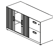
Fixed Return Combination Cabinet w/ Roller Door & 2 Drawers 固定组合边柜，卷门及两斗抽屉 W800 - W1600 x D450 x H710 (except W1300, W1500)
